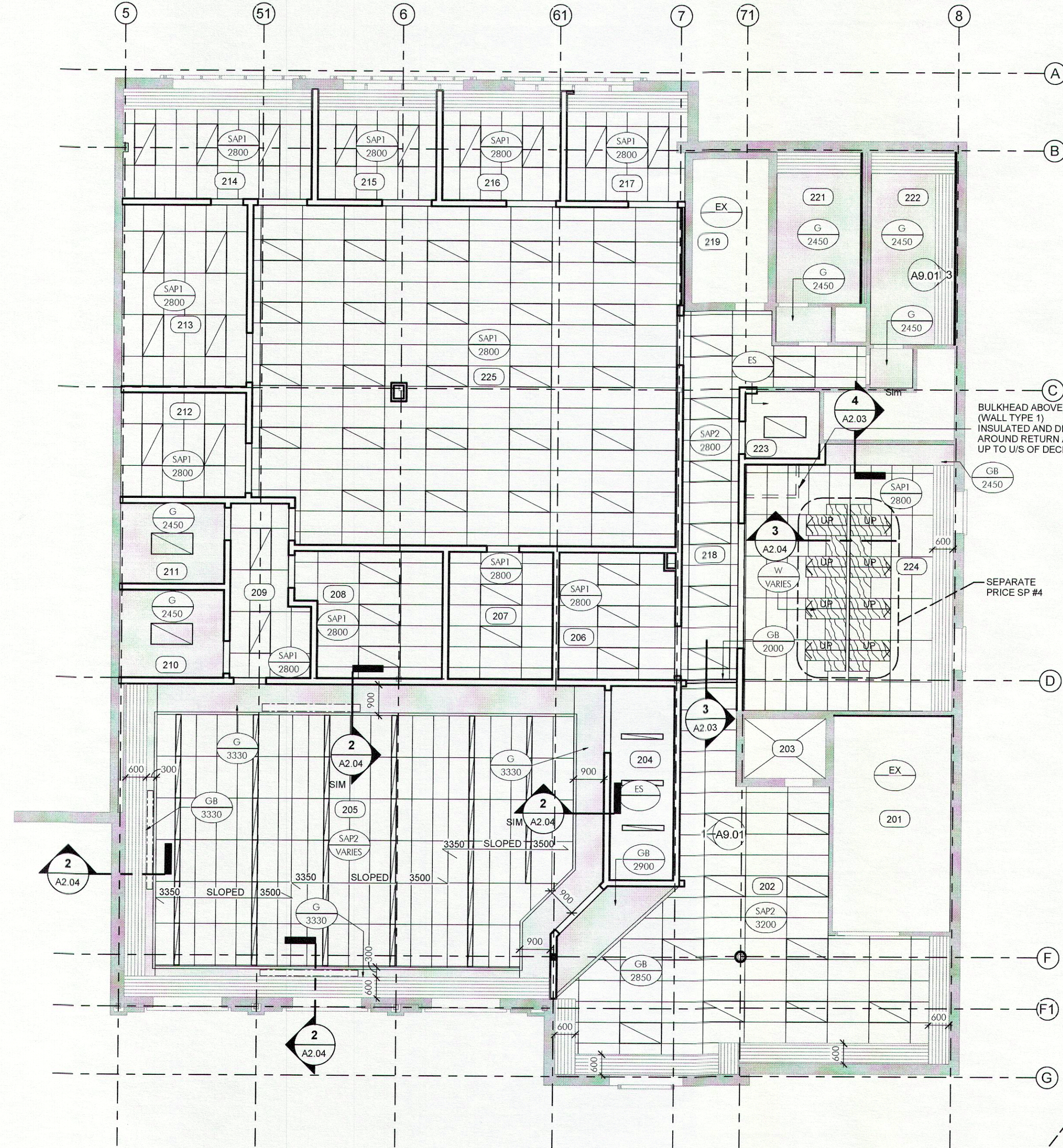
1 2.04 SECOND FLOOR - REFLECTED CEILING PLAN
