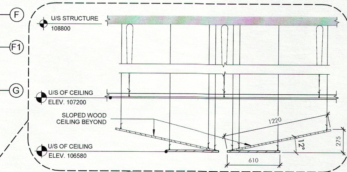
3 BULKHEAD SECTION A2.04 1:25
